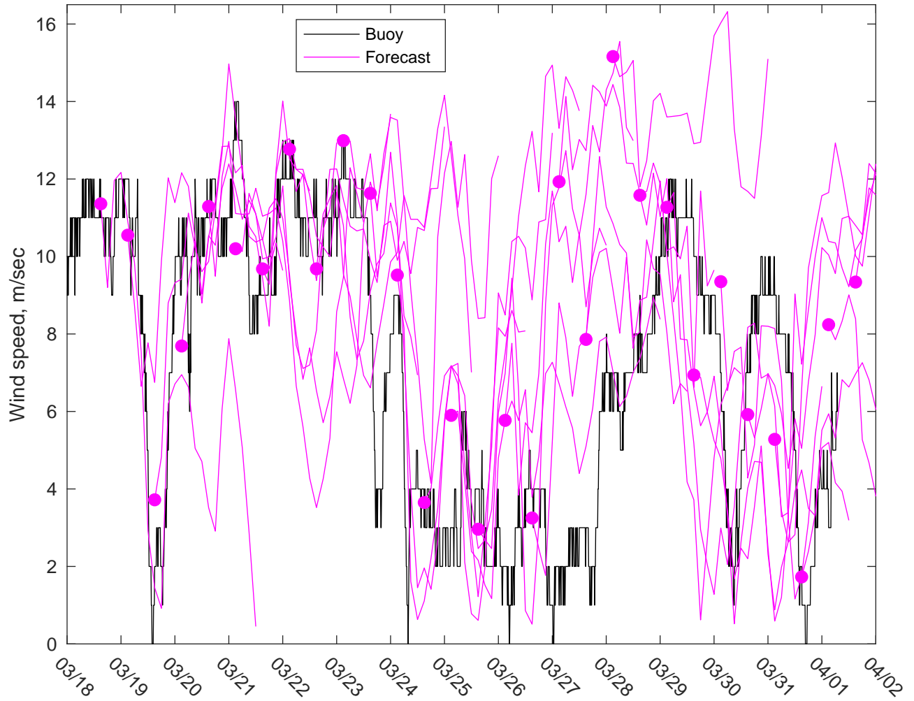
NDBC 46054 vs GFS Winds: 7 to 10 day forecast
