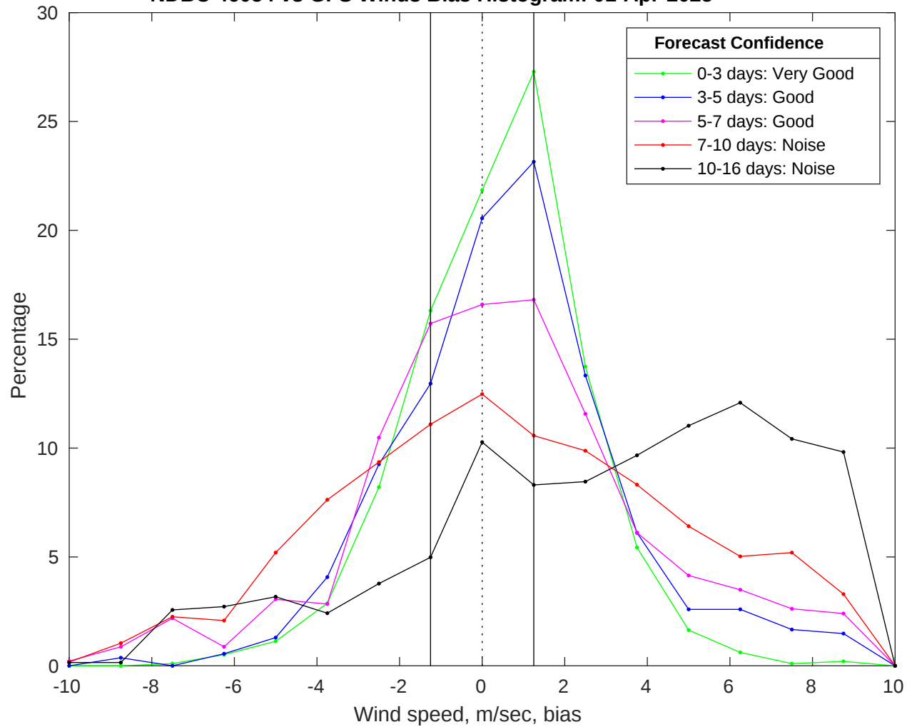
NDBC 46054 vs GFS Winds Bias Histogram: 01-Apr-2025
