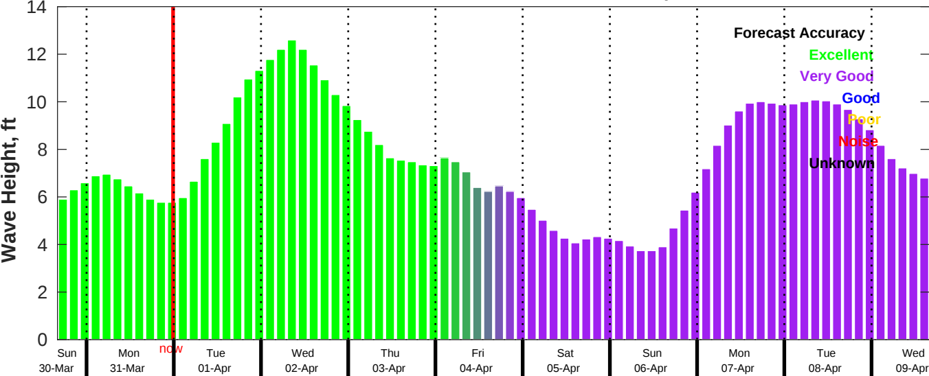
CMEMS Wave Forecast for NDBC 46054 from 30-Mar-2025 16:00:00 to 09-Apr-2025 16:00:00
