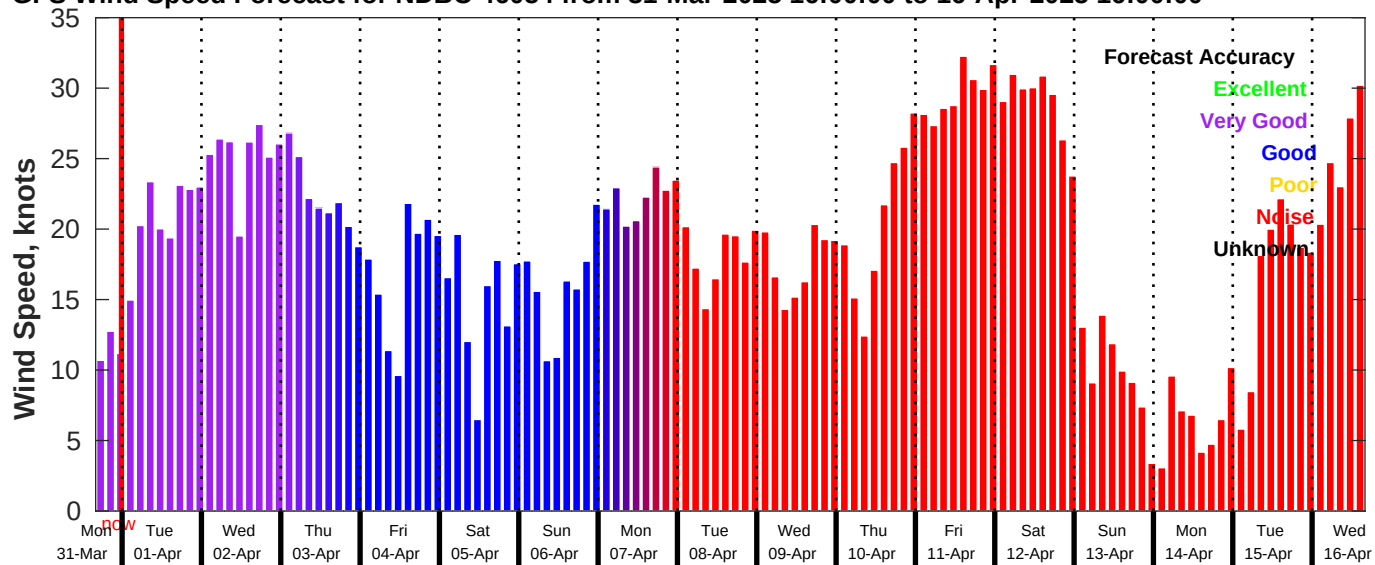
GFS Wind Speed Forecast for NDBC 46054 from 31-Mar-2025 16:00:00 to 16-Apr-2025 16:00:00
