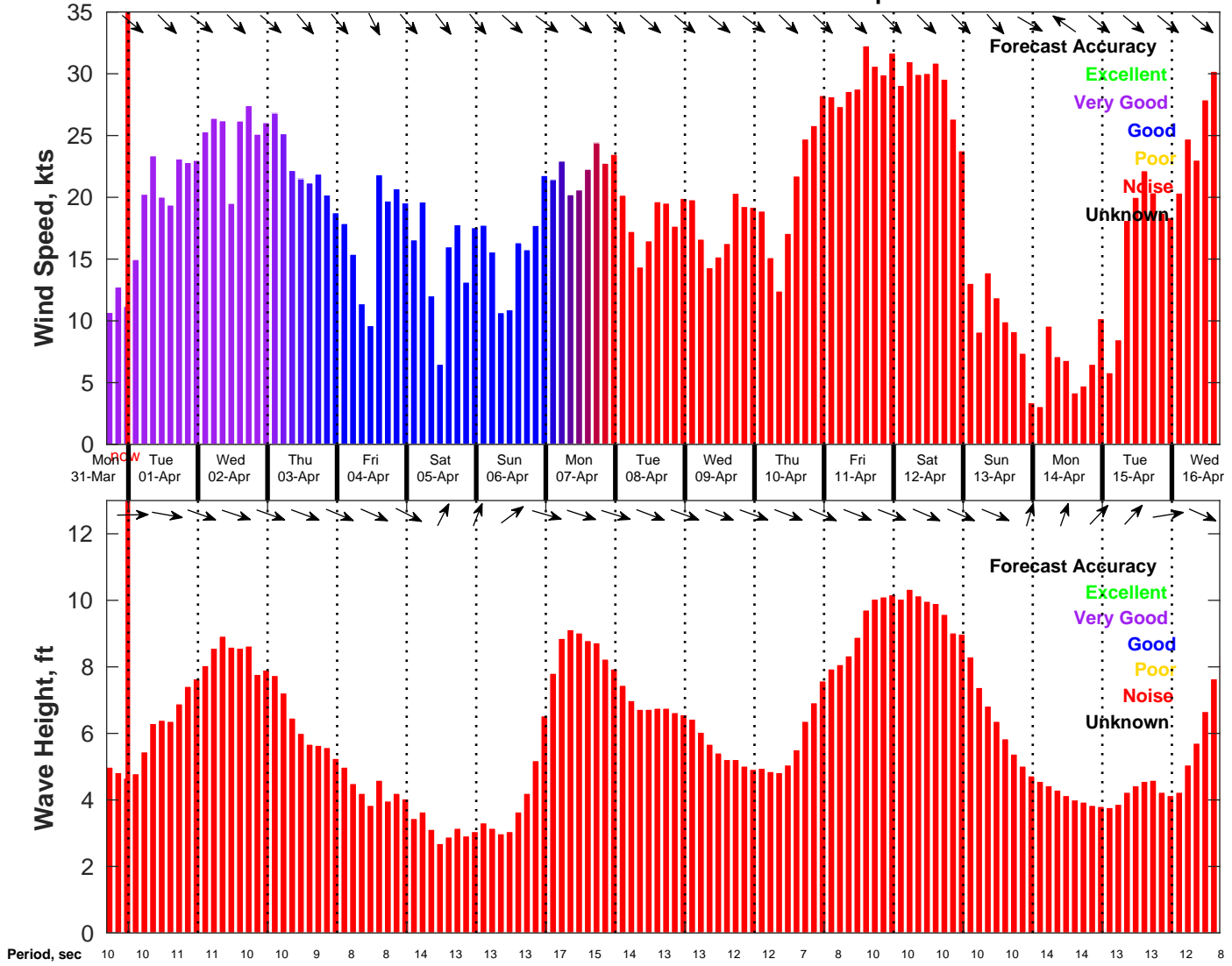
Wind & Wave Forecast for NDBC 46054 from 31-Mar-2025 16:00:00 to 16-Apr-2025 16:00:00
