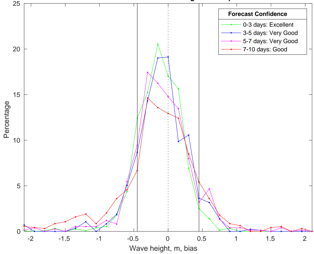
NDBC 46069 vs CMEMS Waves Bias Histogram: 01-Apr-2025
