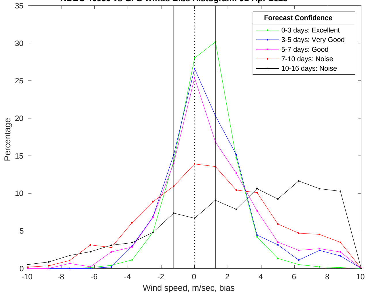
NDBC 46069 vs GFS Winds Bias Histogram: 01-Apr-2025
