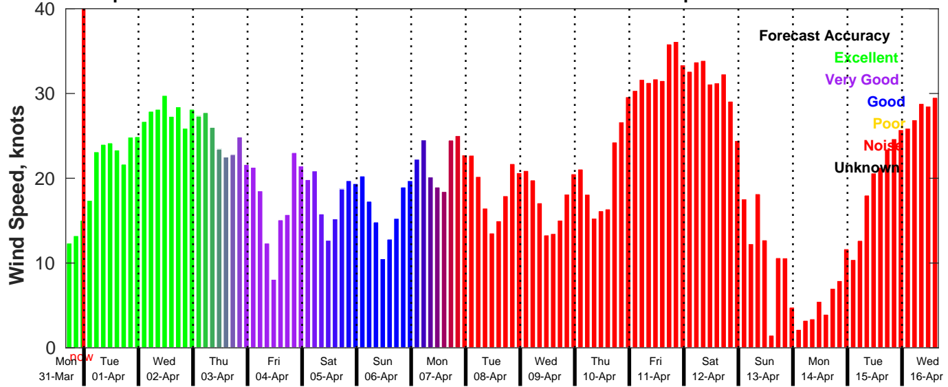
GFS Wind Speed Forecast for NDBC 46069 from 31-Mar-2025 16:00:00 to 16-Apr-2025 16:00:00
