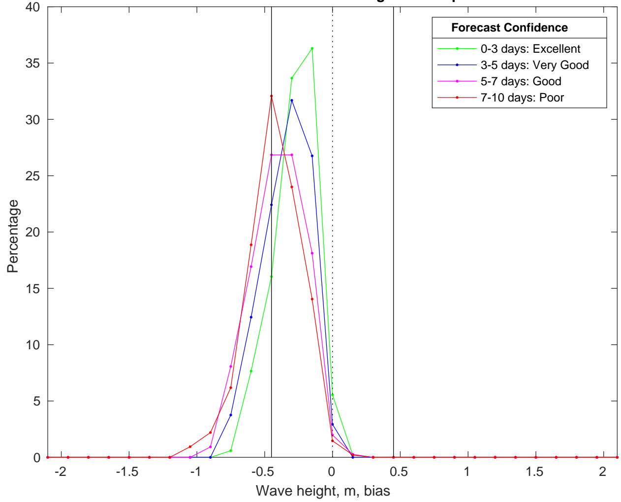
NDBC 51209 vs CMEMS Waves Bias Histogram: 01-Apr-2025
