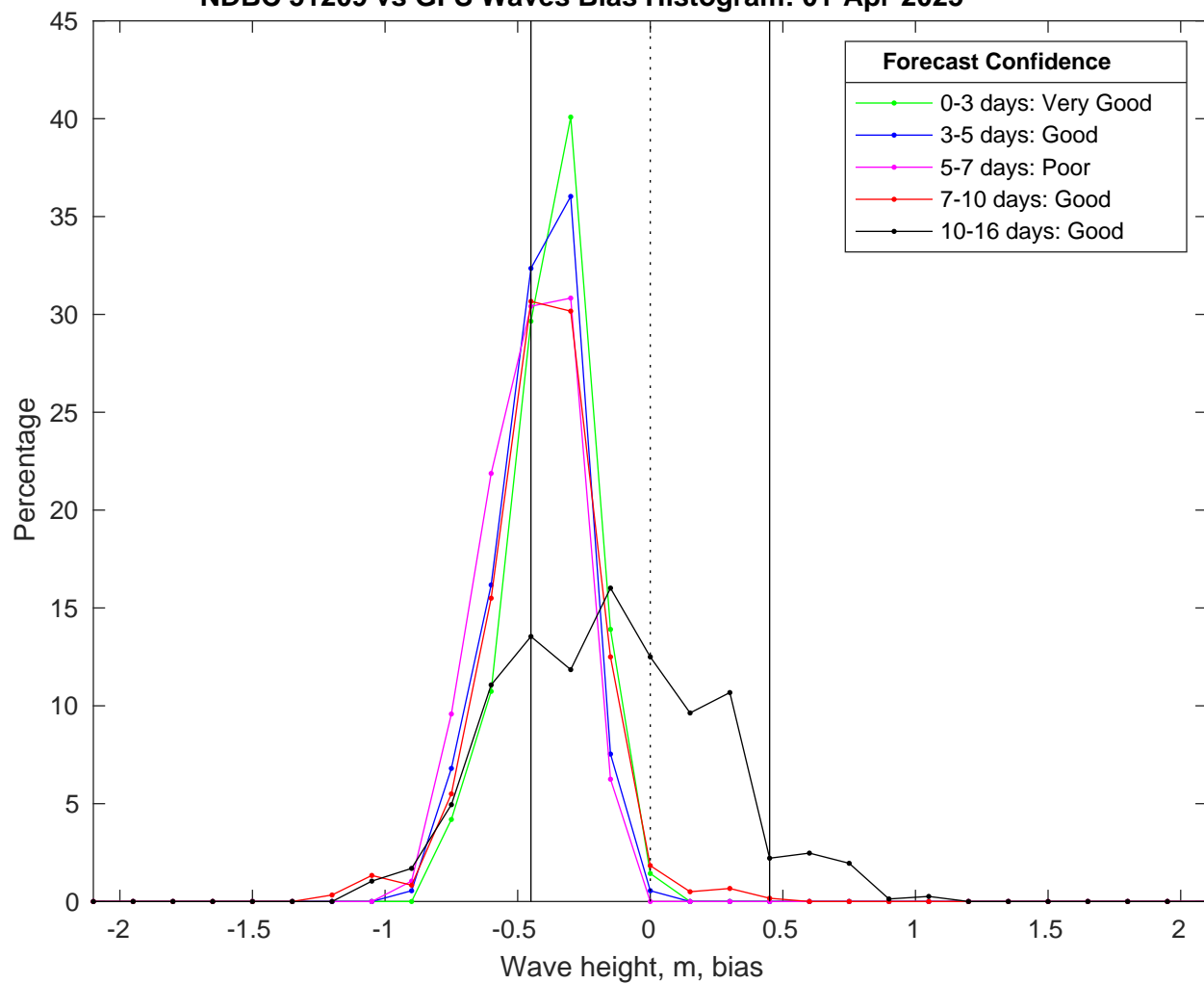
NDBC 51209 vs GFS Waves Bias Histogram: 01-Apr-2025
