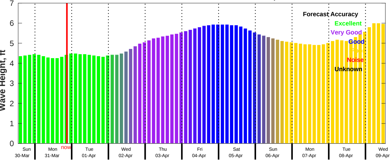
CMEMS Wave Forecast for NDBC 51209 from 30-Mar-2025 13:00:00 to 09-Apr-2025 13:00:00
