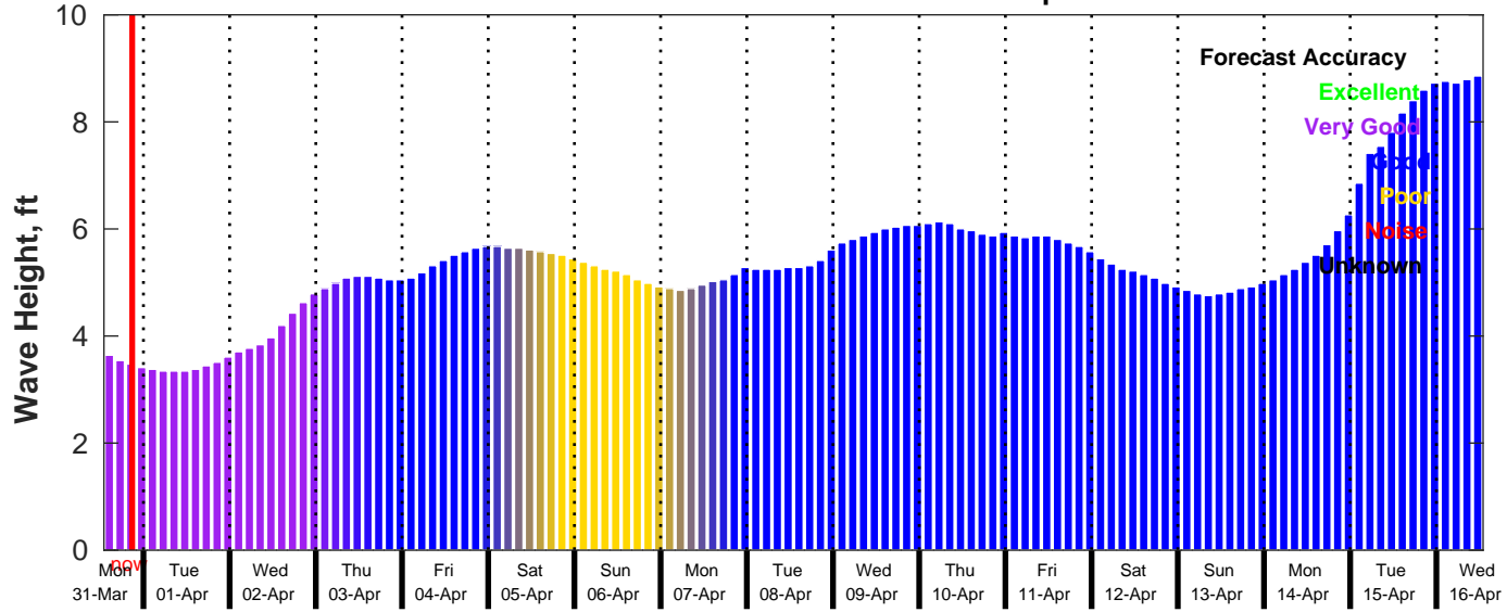
GFS Wave Forecast for NDBC 51209 from 31-Mar-2025 13:00:00 to 16-Apr-2025 13:00:00
