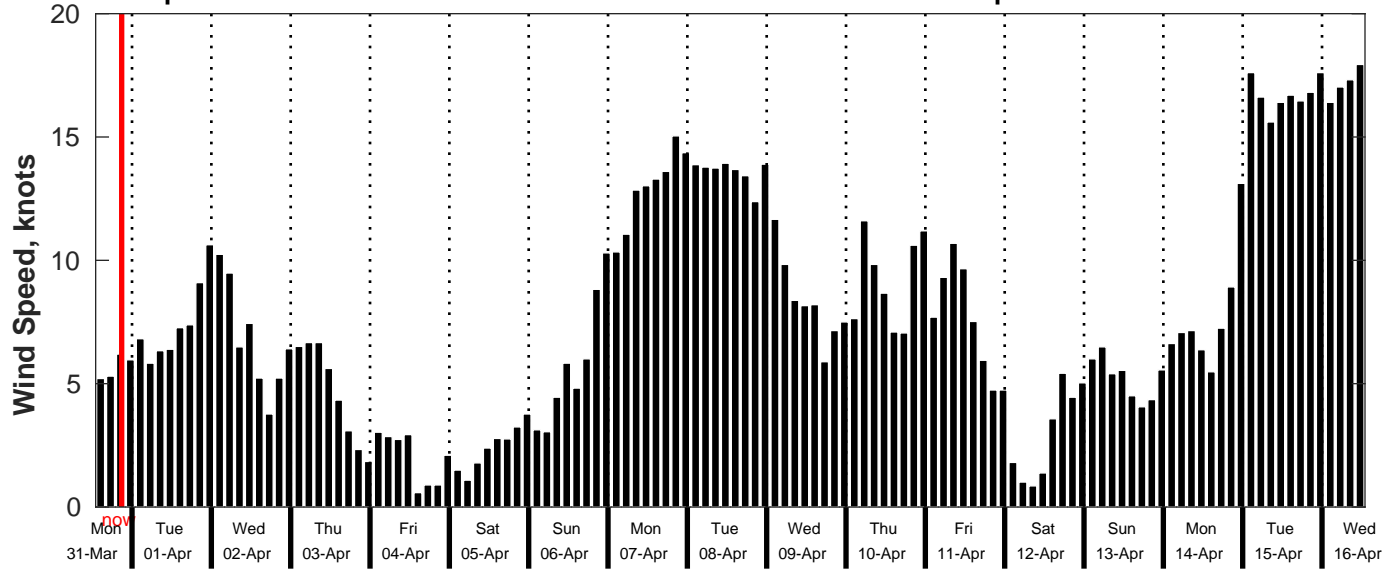
GFS Wind Speed Forecast for NDBC 51209 from 31-Mar-2025 13:00:00 to 16-Apr-2025 13:00:00
