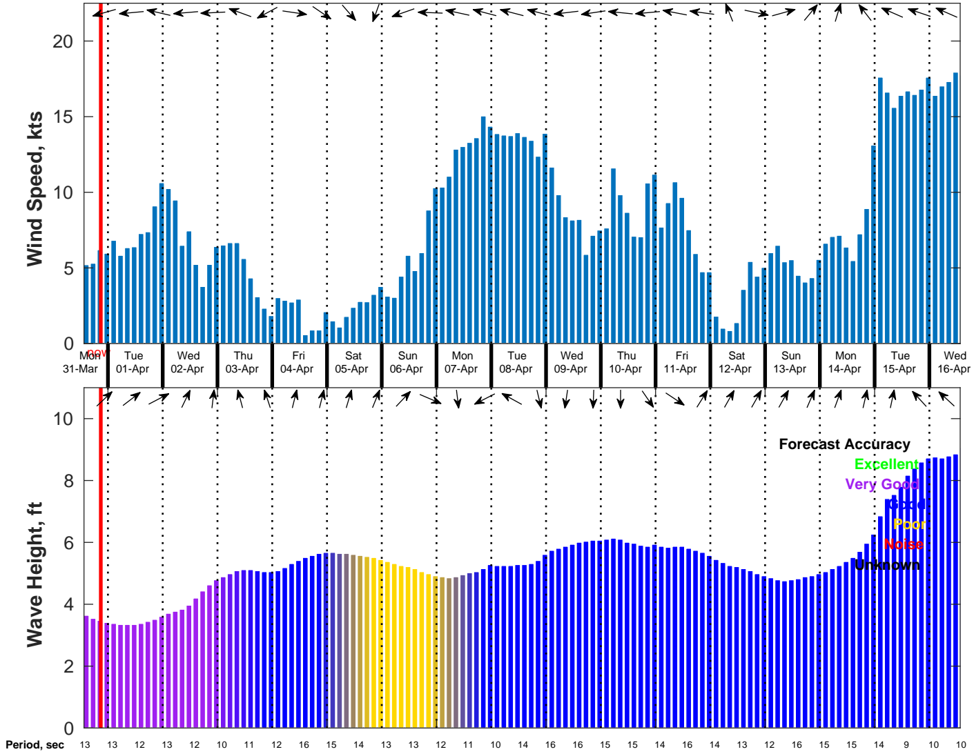
Wind & Wave Forecast for NDBC 51209 from 31-Mar-2025 13:00:00 to 16-Apr-2025 13:00:00
