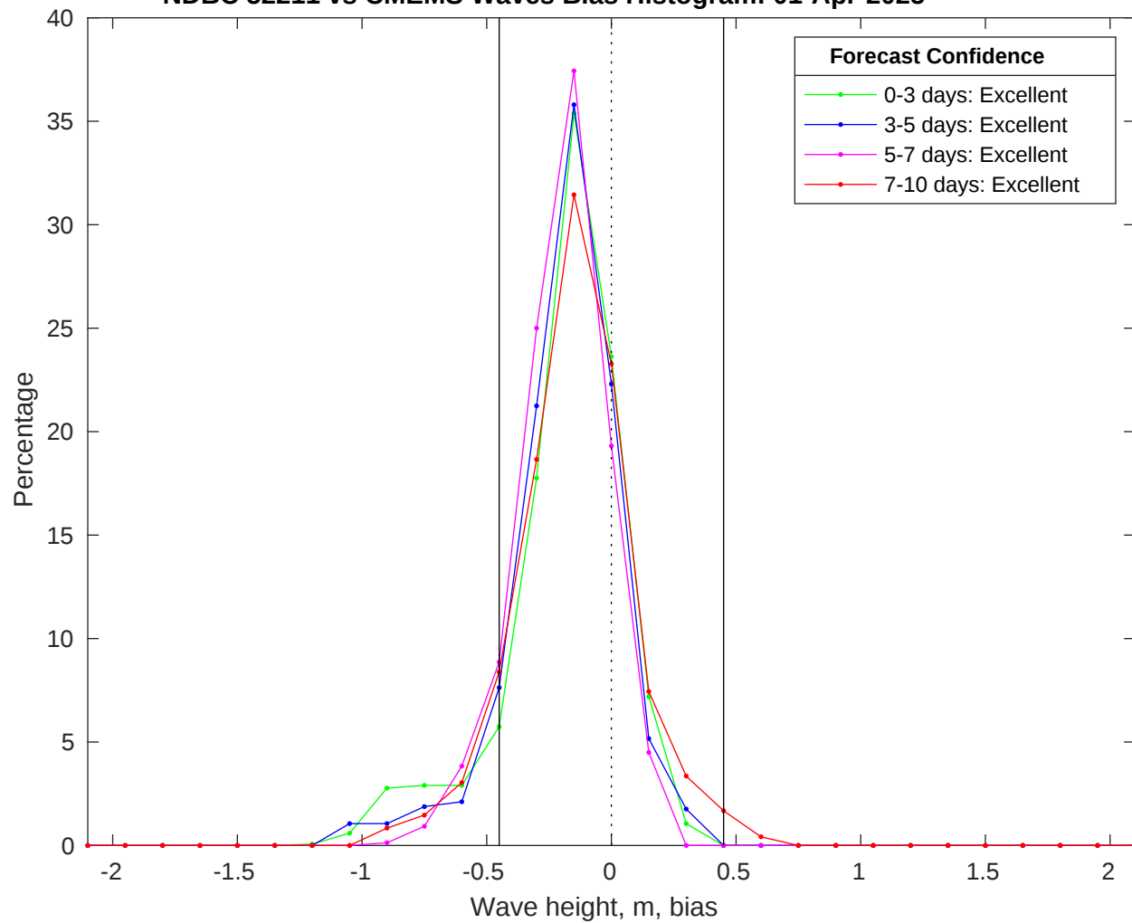
NDBC 52211 vs CMEMS Waves Bias Histogram: 01-Apr-2025
