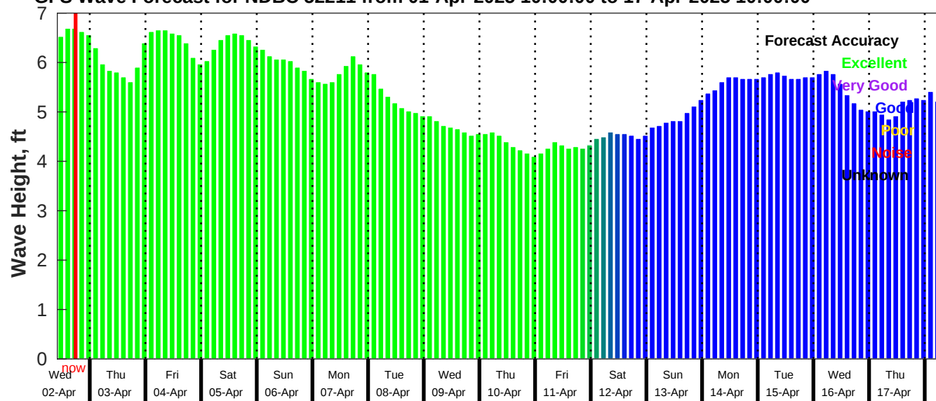
GFS Wave Forecast for NDBC 52211 from 01-Apr-2025 10:00:00 to 17-Apr-2025 10:00:00
