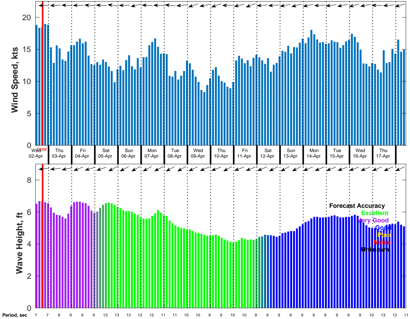
Wind & Wave Forecast for NDBC 52211 from 01-Apr-2025 10:00:00 to 17-Apr-2025 10:00:00
