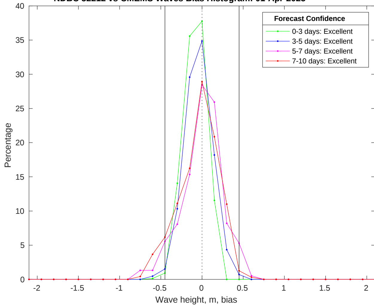
NDBC 52212 vs CMEMS Waves Bias Histogram: 01-Apr-2025
