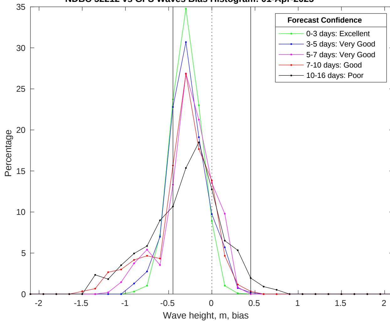
NDBC 52212 vs GFS Waves Bias Histogram: 01-Apr-2025
