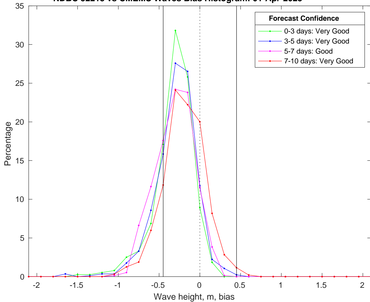
NDBC 52213 vs CMEMS Waves Bias Histogram: 01-Apr-2025
