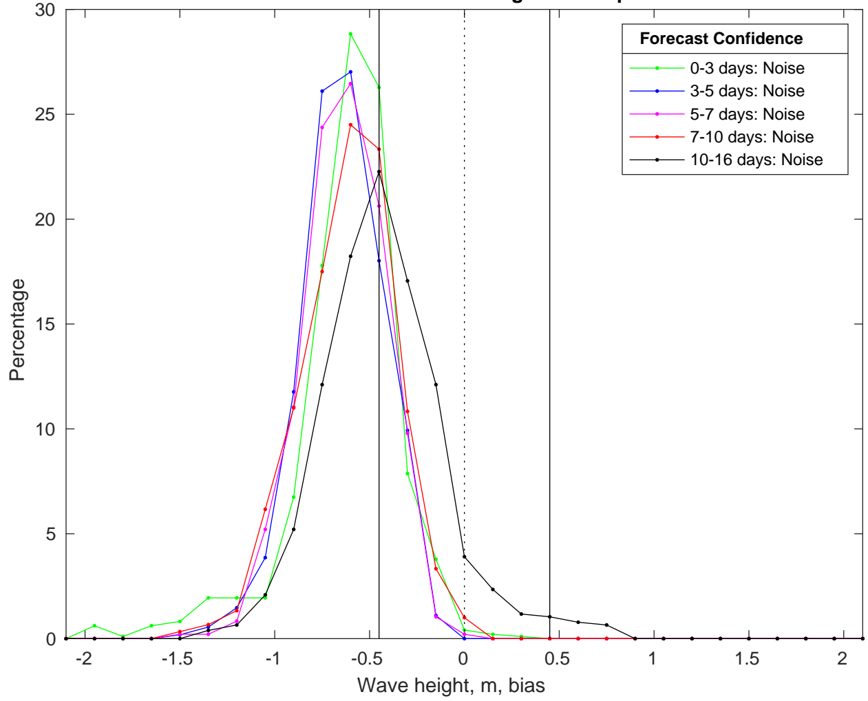
NDBC 52213 vs GFS Waves Bias Histogram: 01-Apr-2025
