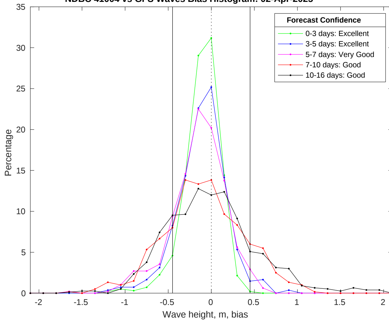
NDBC 41004 vs GFS Waves Bias Histogram: 02-Apr-2025
