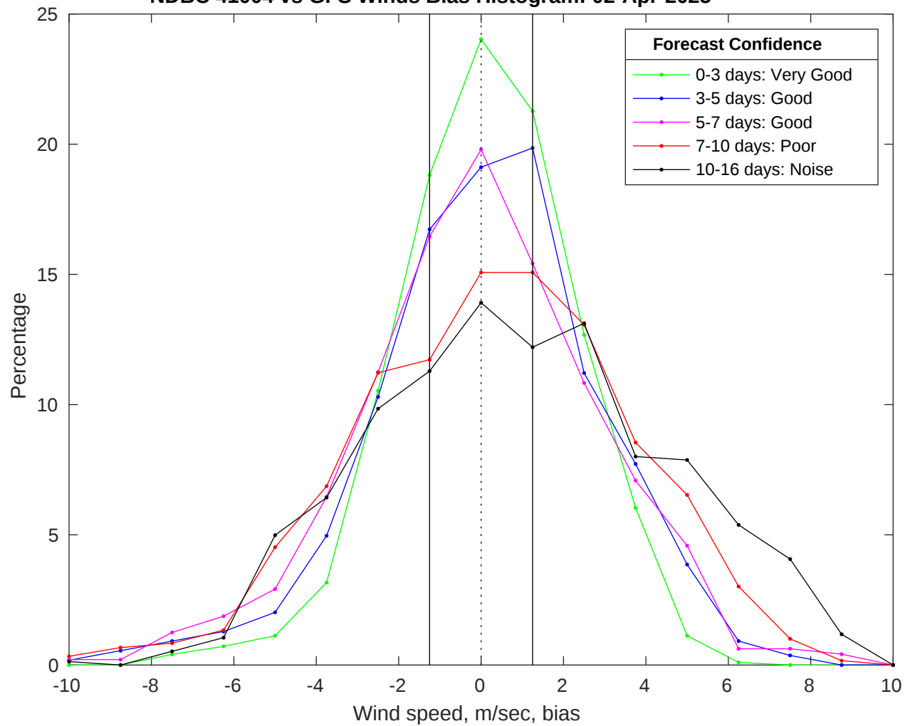
NDBC 41004 vs GFS Winds Bias Histogram: 02-Apr-2025
