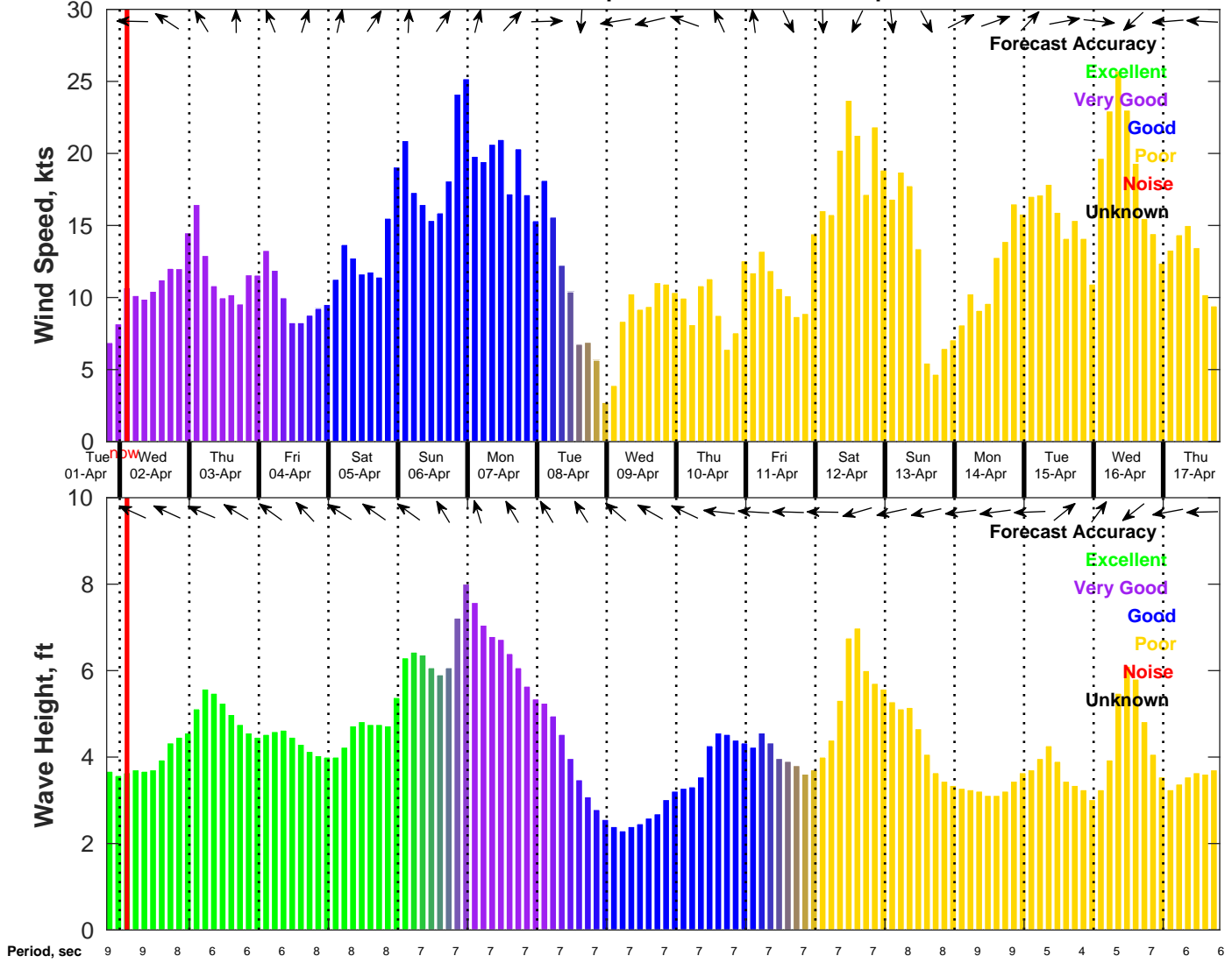
Wind & Wave Forecast for NDBC 41004 from 01-Apr-2025 19:00:00 to 17-Apr-2025 19:00:00
