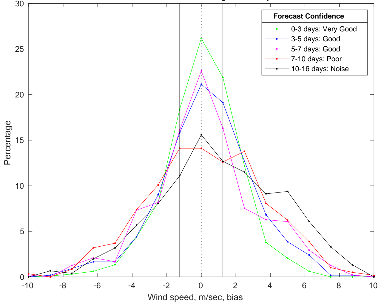
NDBC 41013 vs GFS Winds Bias Histogram: 02-Apr-2025
