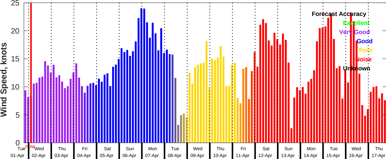
GFS Wind Speed Forecast for NDBC 41013 from 01-Apr-2025 19:00:00 to 17-Apr-2025 19:00:00
