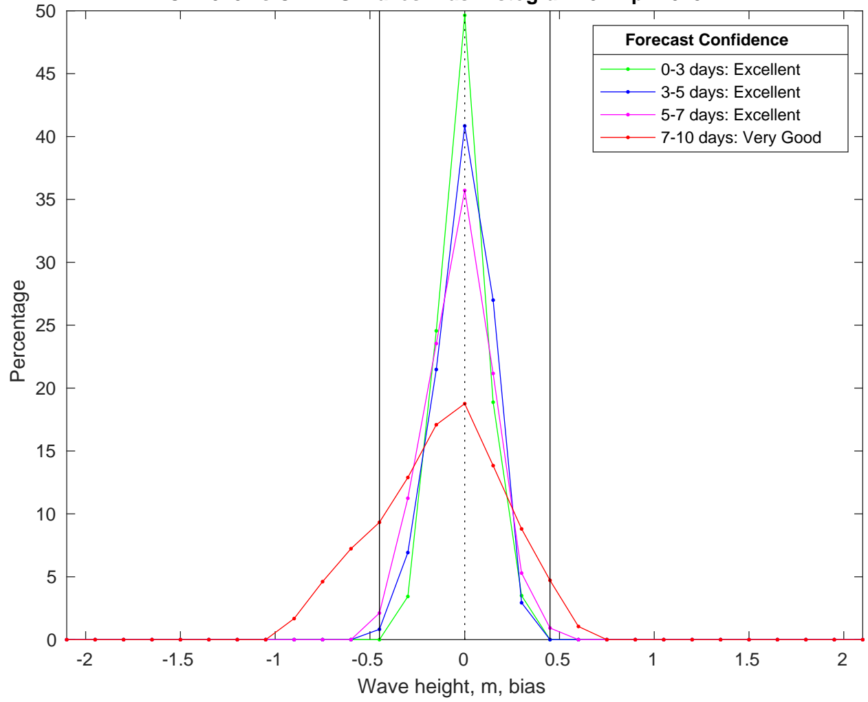
NDBC 41040 vs CMEMS Waves Bias Histogram: 02-Apr-2025
