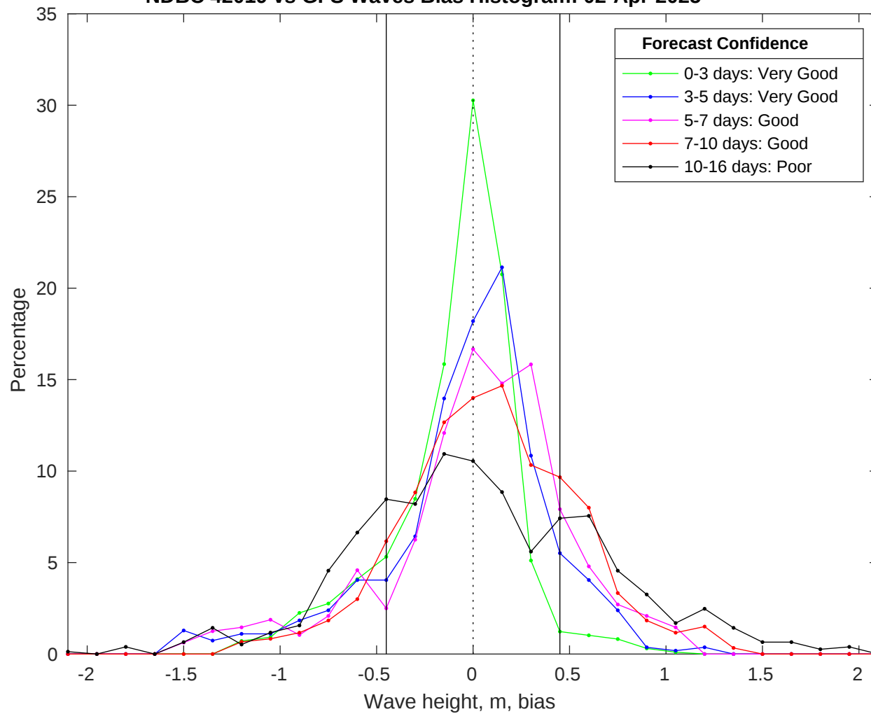
NDBC 42019 vs GFS Waves Bias Histogram: 02-Apr-2025
