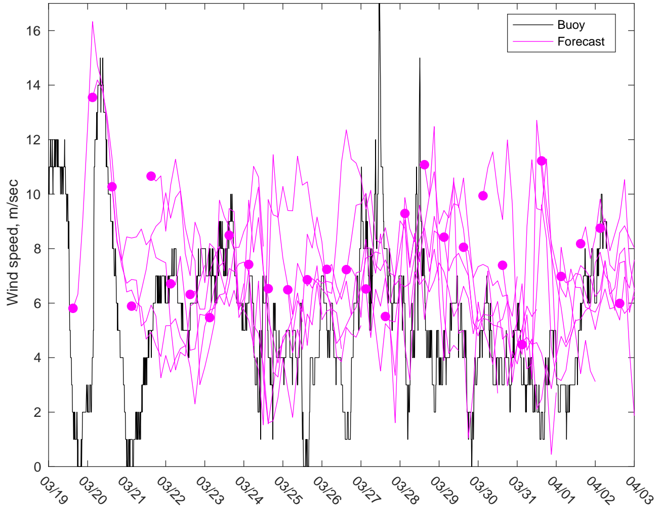
NDBC 42019 vs GFS Winds: 7 to 10 day forecast
