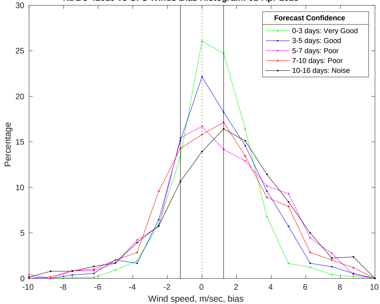
NDBC 42019 vs GFS Winds Bias Histogram: 02-Apr-2025
