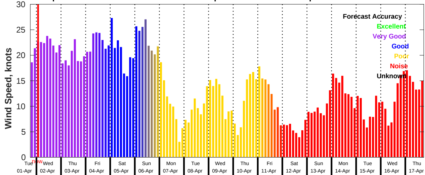
GFS Wind Speed Forecast for NDBC 42019 from 01-Apr-2025 18:00:00 to 17-Apr-2025 18:00:00
