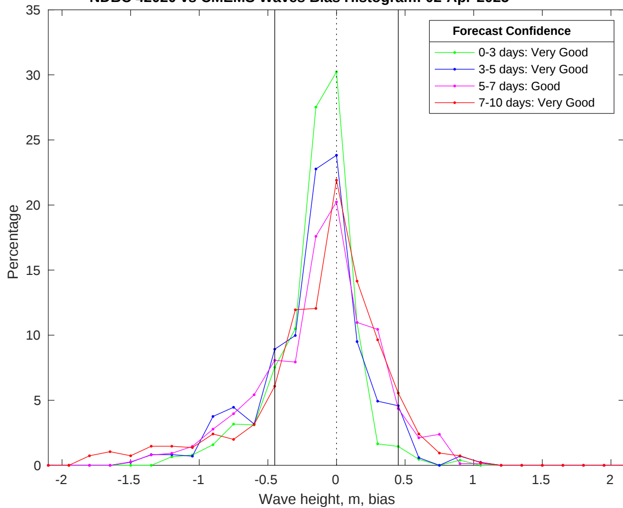
NDBC 42020 vs CMEMS Waves Bias Histogram: 02-Apr-2025
