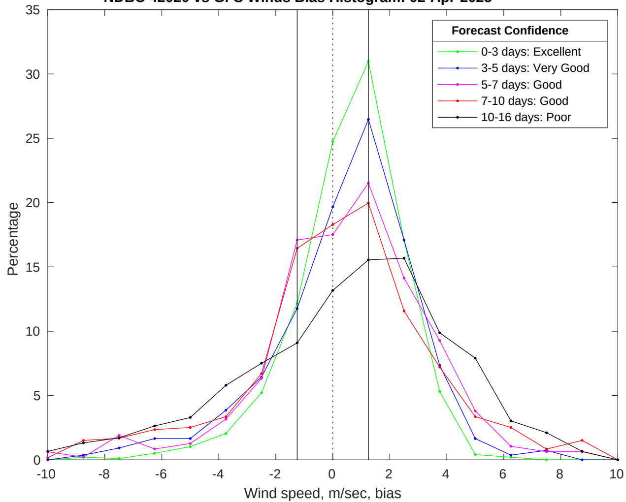
NDBC 42020 vs GFS Winds Bias Histogram: 02-Apr-2025
