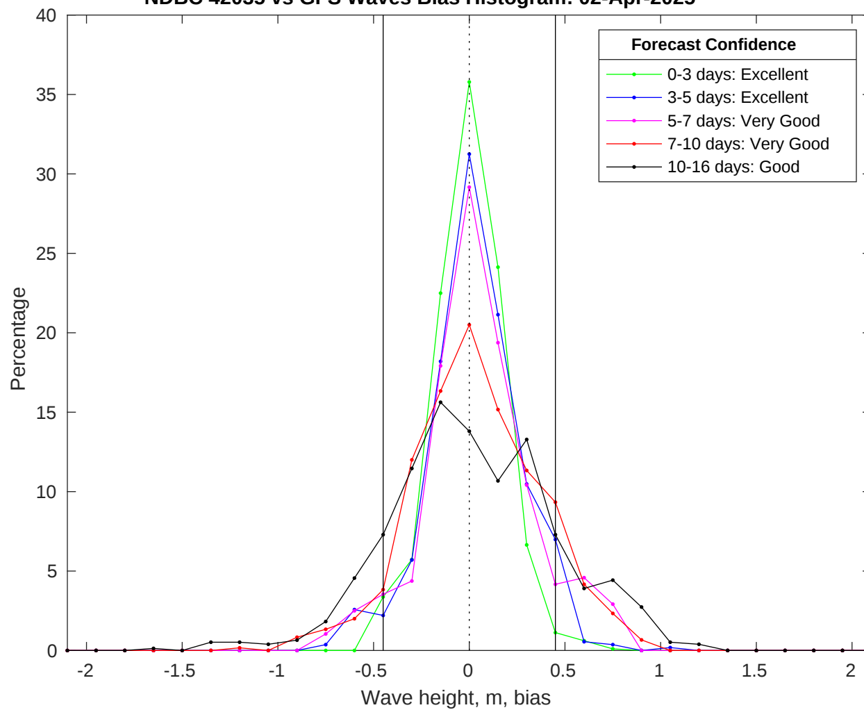
NDBC 42035 vs GFS Waves Bias Histogram: 02-Apr-2025
