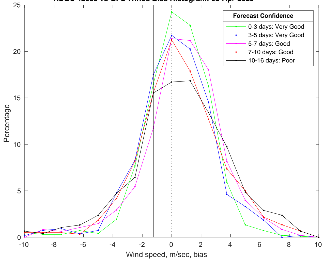
NDBC 42035 vs GFS Winds Bias Histogram: 02-Apr-2025
