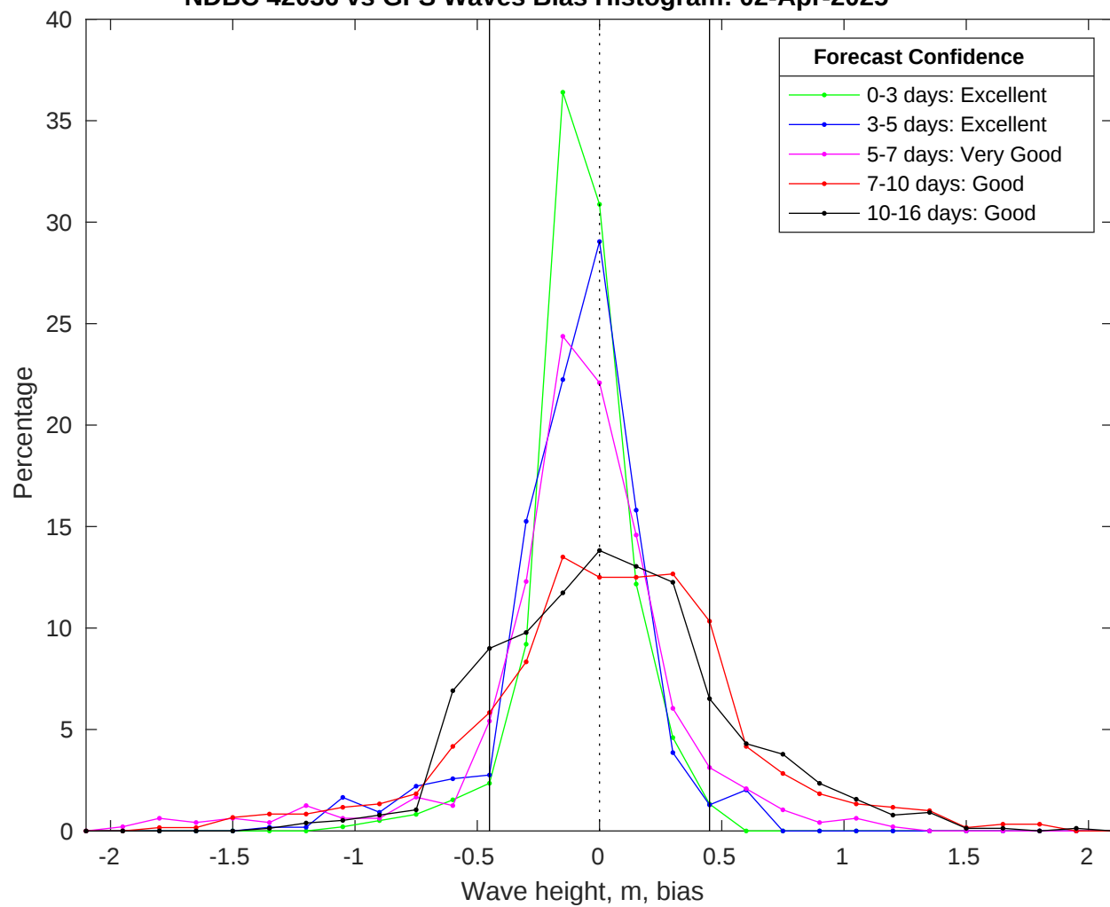
NDBC 42036 vs GFS Waves Bias Histogram: 02-Apr-2025
