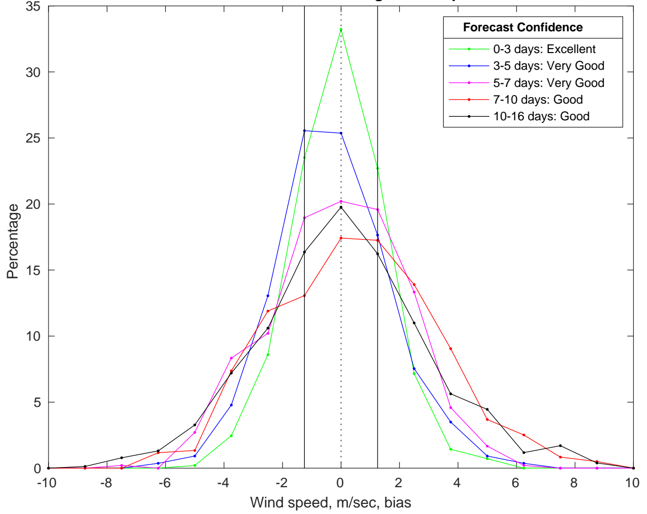
NDBC 42036 vs GFS Winds Bias Histogram: 02-Apr-2025
