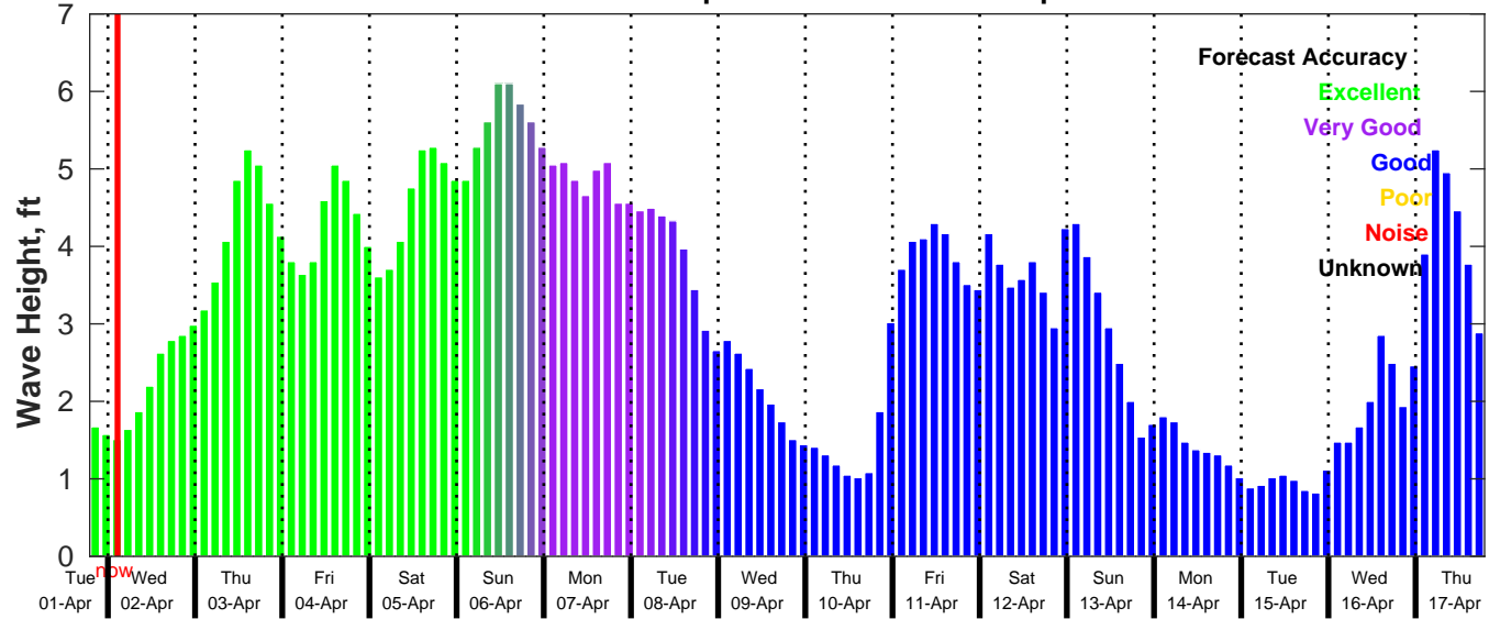
GFS Wave Forecast for NDBC 42036 from 01-Apr-2025 19:00:00 to 17-Apr-2025 19:00:00
