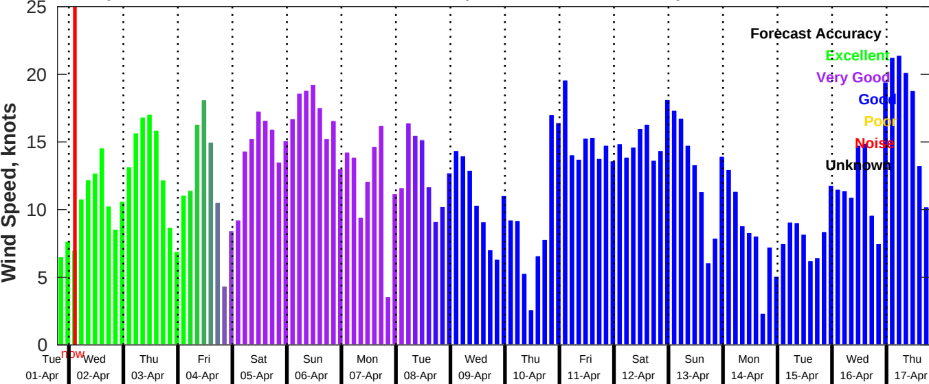
GFS Wind Speed Forecast for NDBC 42036 from 01-Apr-2025 19:00:00 to 17-Apr-2025 19:00:00
