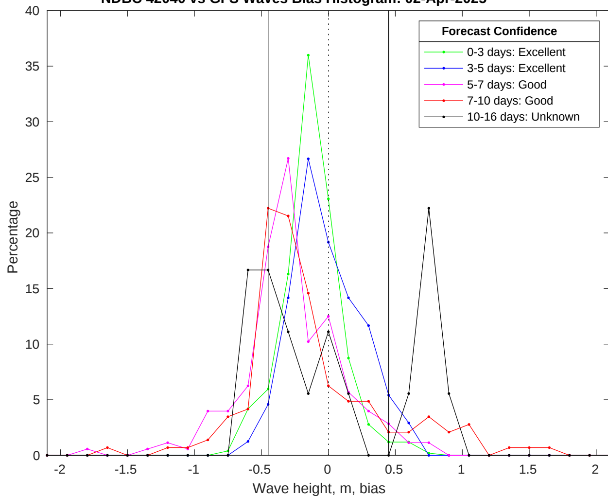
NDBC 42040 vs GFS Waves Bias Histogram: 02-Apr-2025
