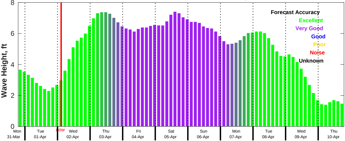
CMEMS Wave Forecast for NDBC 42040 from 31-Mar-2025 19:00:00 to 10-Apr-2025 19:00:00
