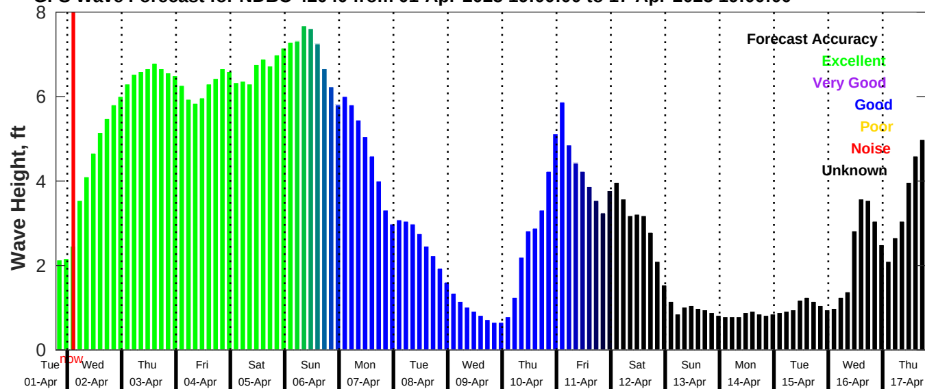
GFS Wave Forecast for NDBC 42040 from 01-Apr-2025 19:00:00 to 17-Apr-2025 19:00:00
