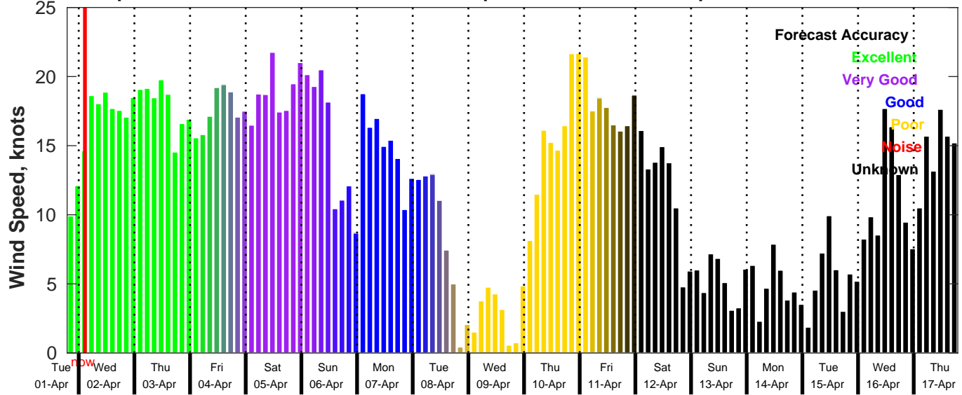
GFS Wind Speed Forecast for NDBC 42040 from 01-Apr-2025 19:00:00 to 17-Apr-2025 19:00:00
