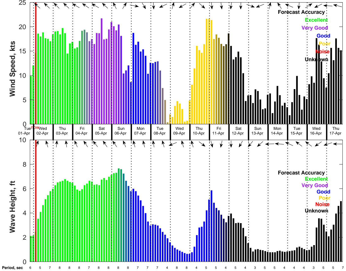
Wind & Wave Forecast for NDBC 42040 from 01-Apr-2025 19:00:00 to 17-Apr-2025 19:00:00
