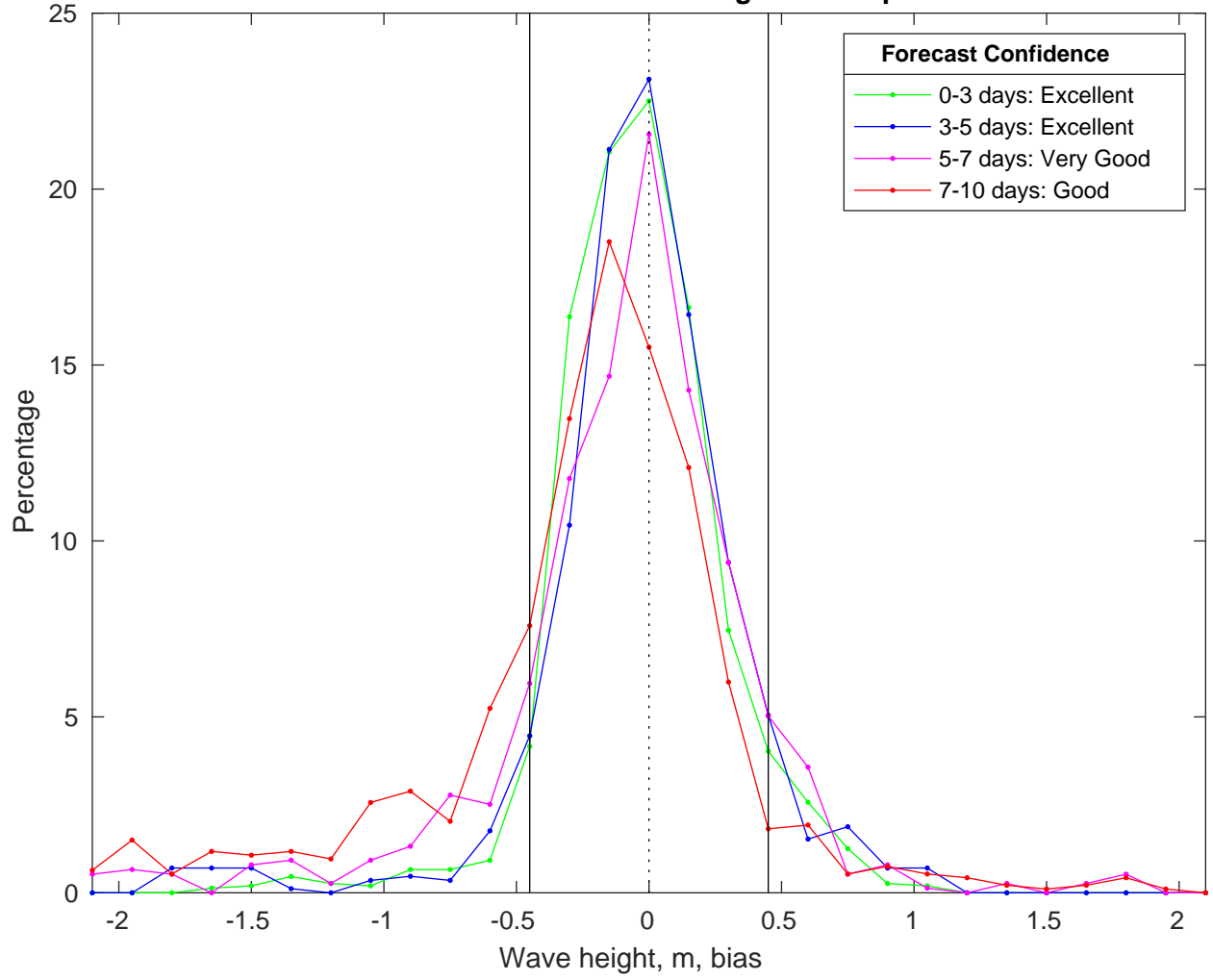
NDBC 46011 vs CMEMS Waves Bias Histogram: 02-Apr-2025
