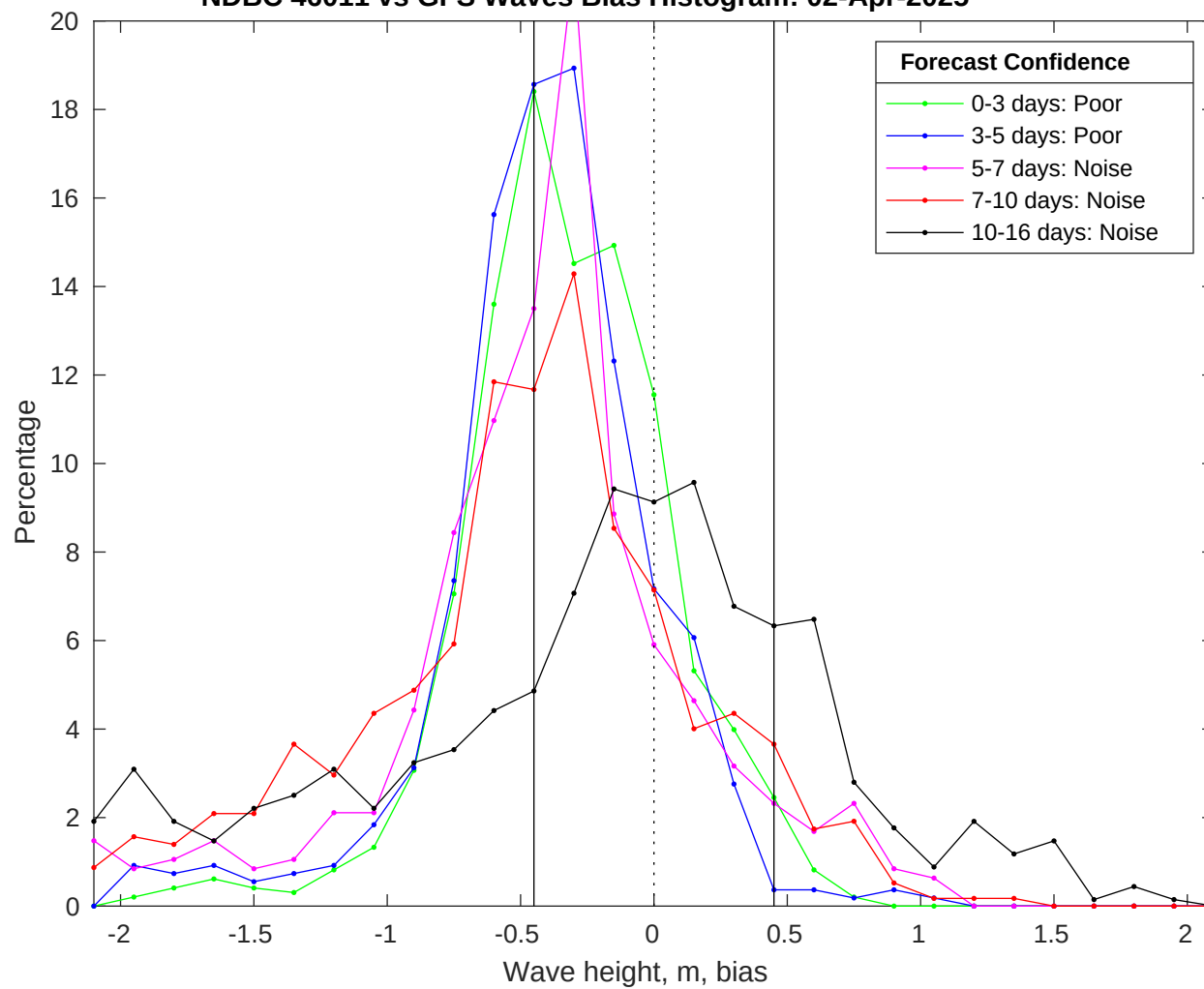
NDBC 46011 vs GFS Waves Bias Histogram: 02-Apr-2025
