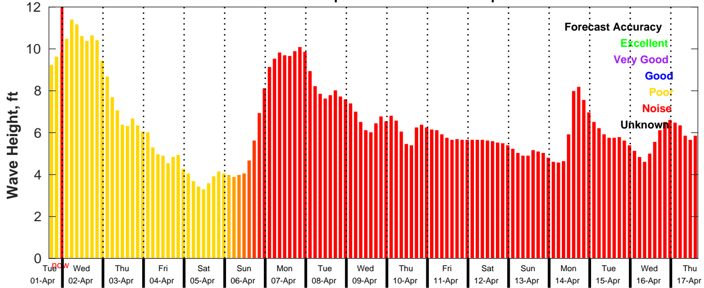
GFS Wave Forecast for NDBC 46011 from 01-Apr-2025 16:00:00 to 17-Apr-2025 16:00:00
