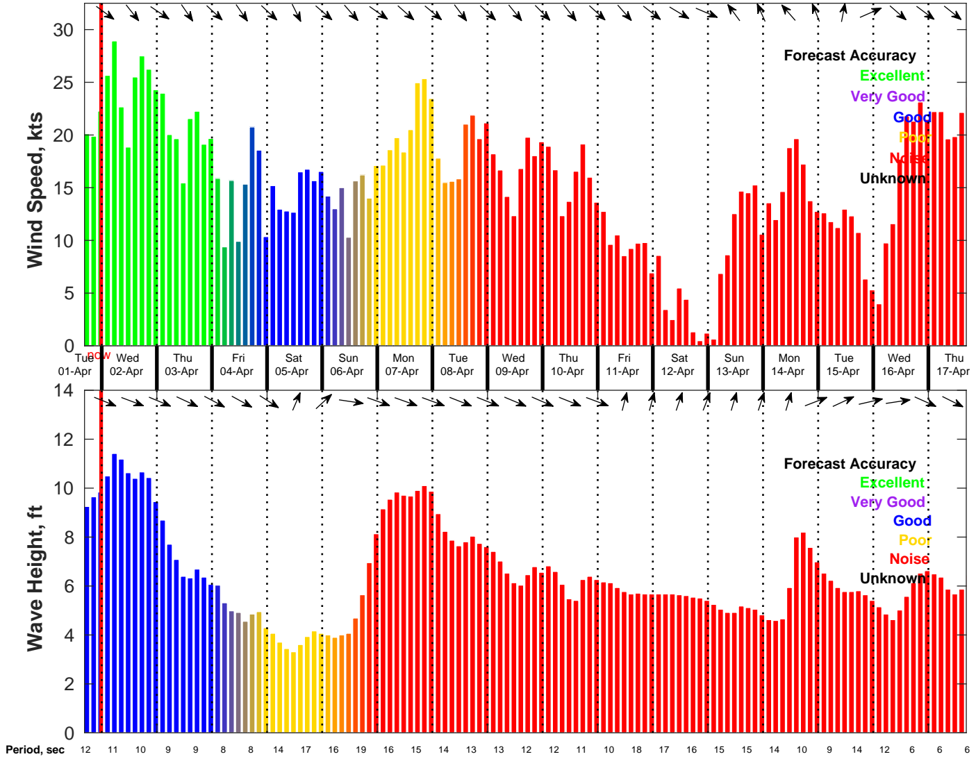
Wind & Wave Forecast for NDBC 46011 from 01-Apr-2025 16:00:00 to 17-Apr-2025 16:00:00
