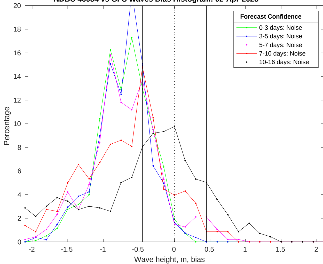
NDBC 46054 vs GFS Waves Bias Histogram: 02-Apr-2025
