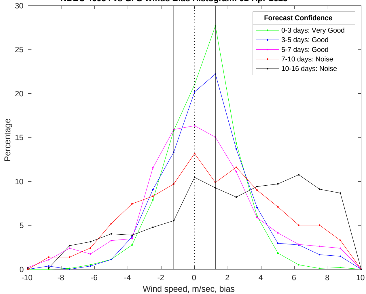
NDBC 46054 vs GFS Winds Bias Histogram: 02-Apr-2025
